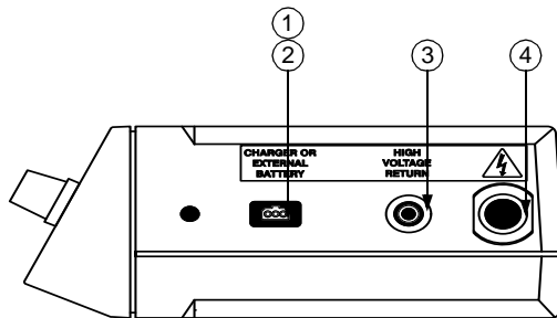
Figure 2. Side connections and terminals layout
