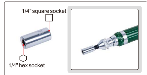
magnetic adapter (included)
