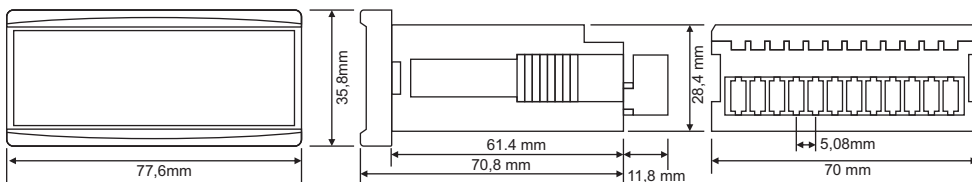
Dimensions for DJ-V36 / DJ-F36
